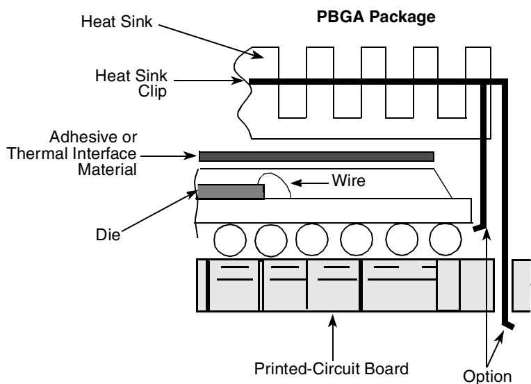
Figure 28. Package Exploded Cross-Sectional View with Several Heat Sink Options
